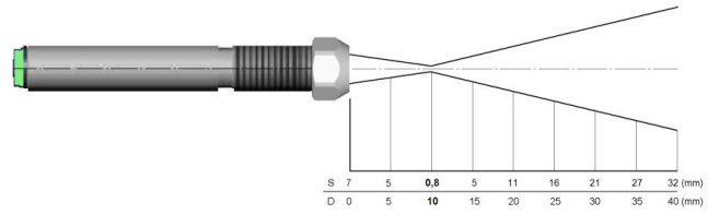
Optical chart: CS (15:1) with CF-lens (0.8mm @ 10mm)
